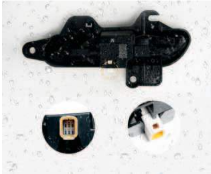
Built-in waterproof rubber ring design IP67 waterproof connector
